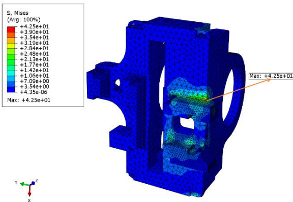
Figure 7: Stress contour for plastic part of blocker-second proposed design
