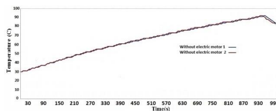
Figure 3: Temperature diagram of the cooling fluid exiting the engine at 1000 rpm in the first and second stages of the test.
