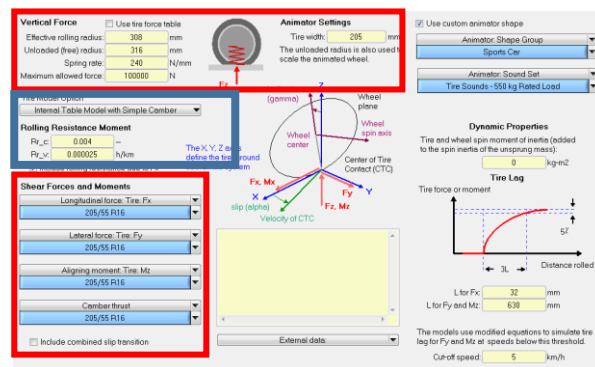
Figure13: CarSim Tire parameters section
