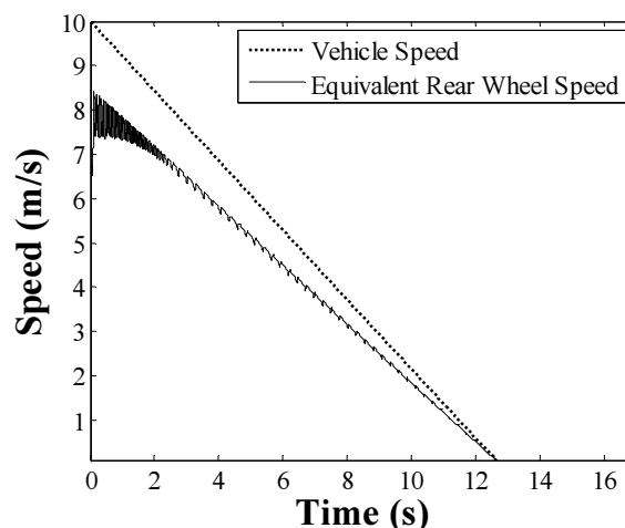
Fig. 13. Vehicle and equivalent rear wheels speed on icy road condition, ARBS
